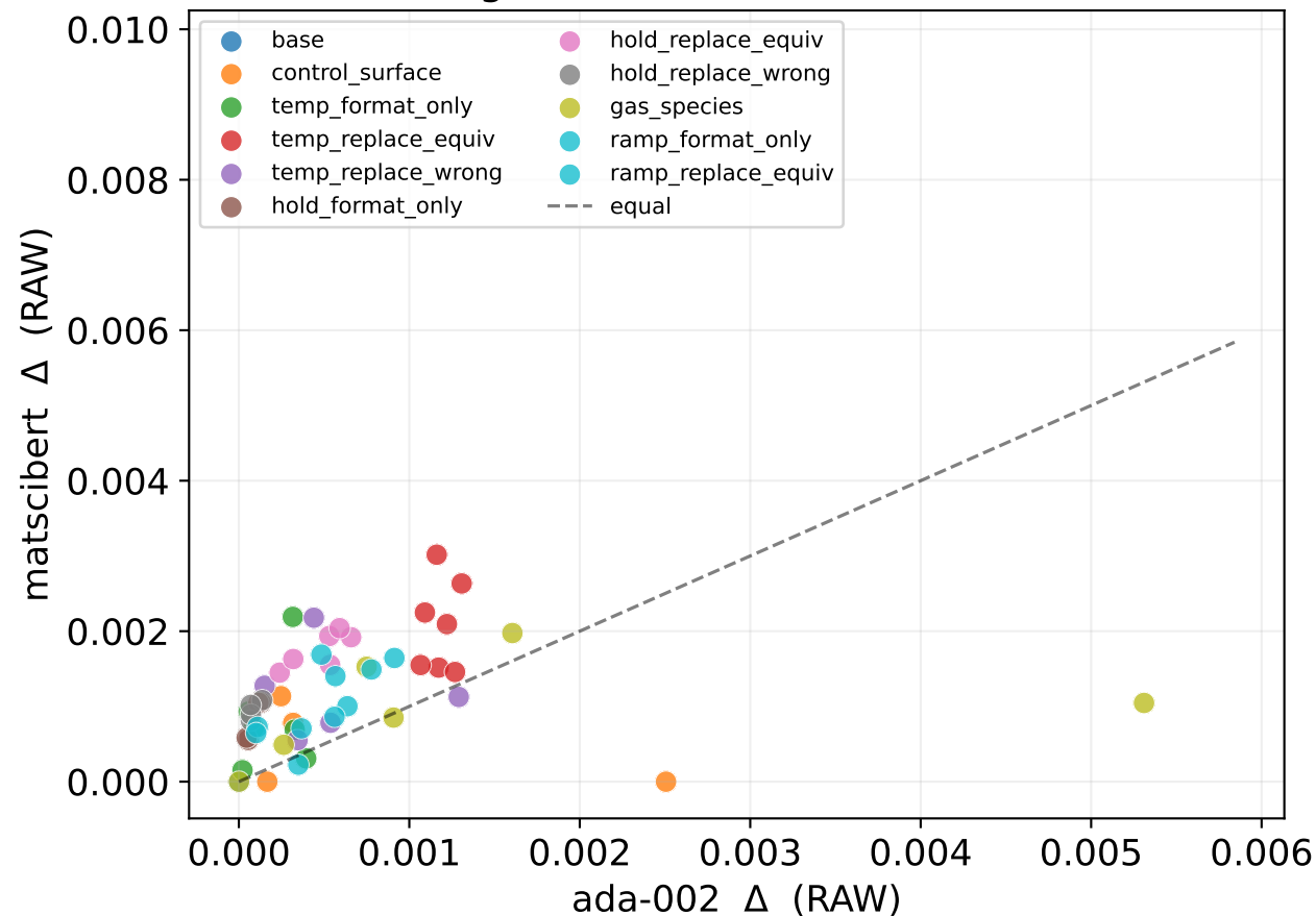
matscibert vs ada-002 above diagonal = matscibert more sensitive
