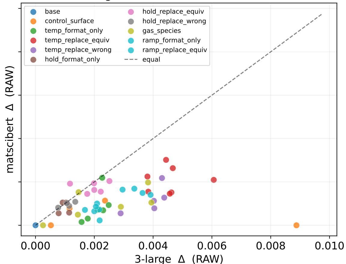
matscibert vs 3-large above diagonal = matscibert more sensitive
